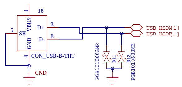
HS USB Device @AP7000
